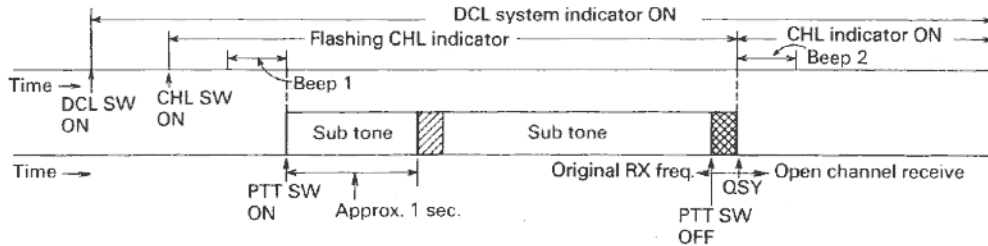
Fig. b. Offset mode (TM-3530A/2570A/2550A/2530A)
