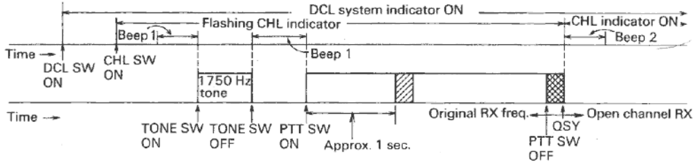
Fig. c. Offset mode (TM-2550E)
